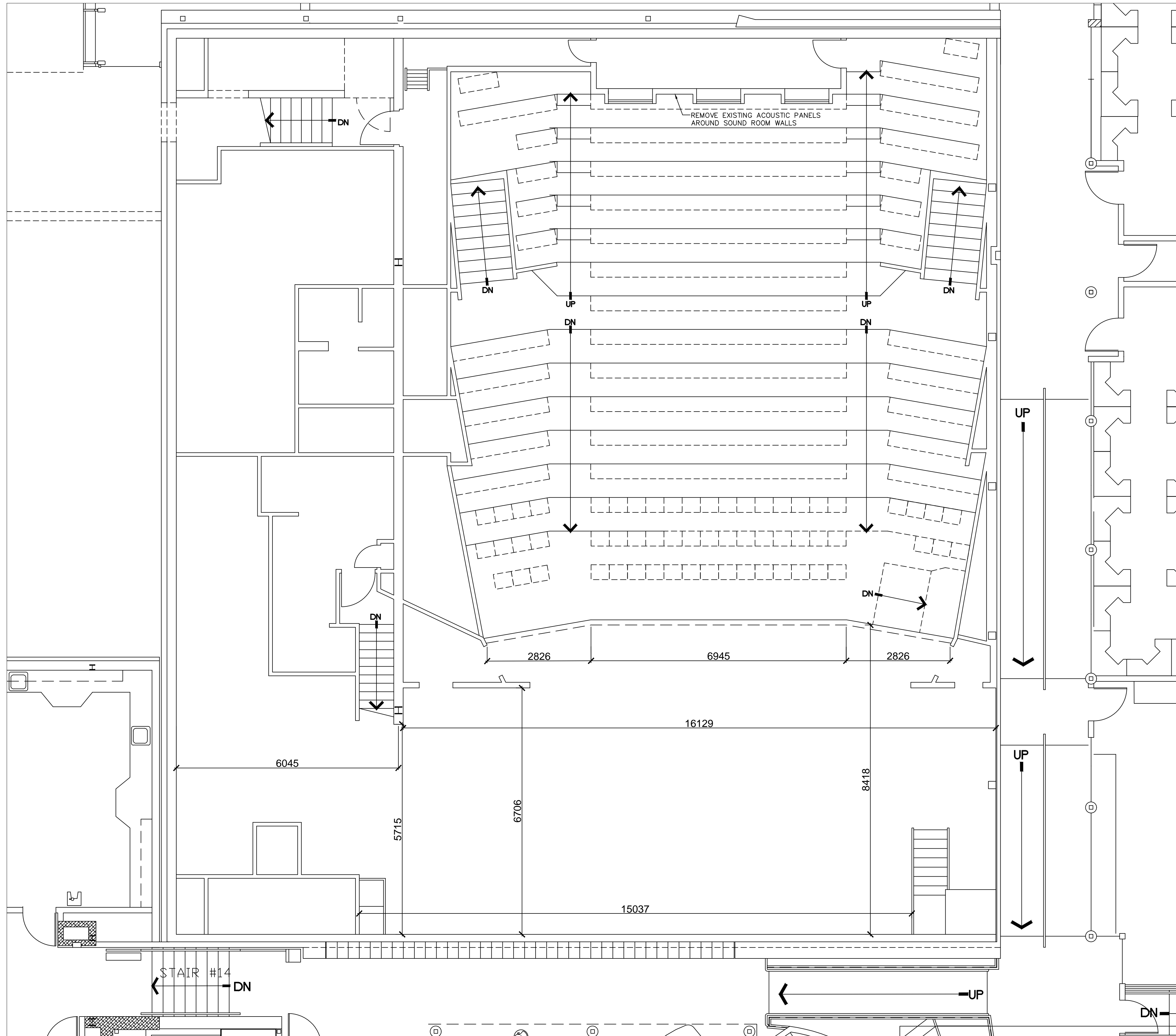
A5 AUDITORIUM FLOOR PLAN - EXISTING M2-01 SCALE: NTS
